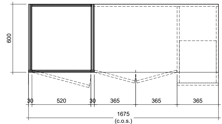
1 - PANTRY DETAIL - PLAN SCALE 1 : 20
