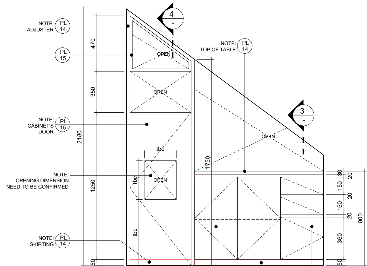
2 - PANTRY DETAIL - ELEV SCALE 1 : 20
