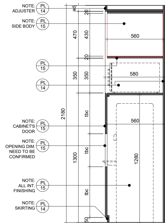
4 - PANTRY-SECT SCALE 1 : 20
